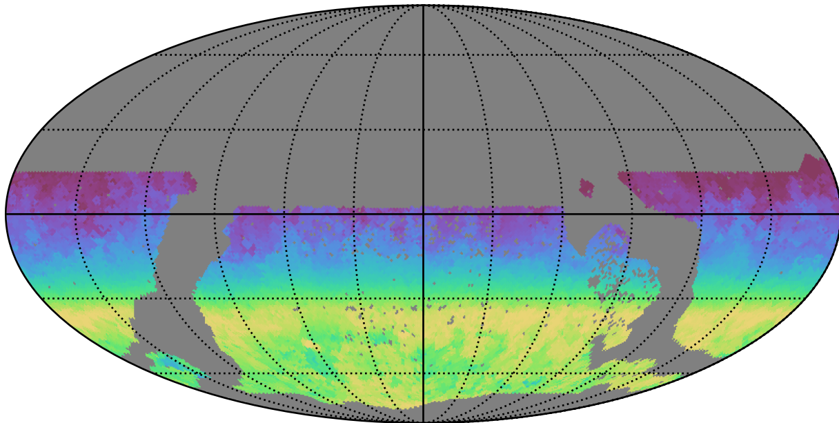
extra_ss_neo7_v3.4_10yrs WFD all bands: AngleRange rotSkyPos
