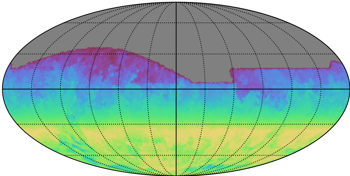
extra_ss_neo7_v3.4_10yrs All sky all bands: AngleRange rotSkyPos
