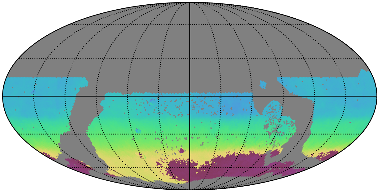
extra_ss_neo7_v3.4_10yrs WFD all bands: AngleMean rotSkyPos
