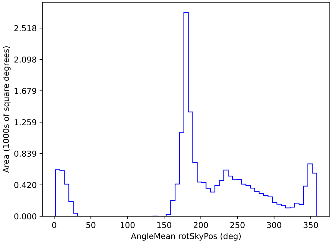
extra_ss_neo7_v3.4_10yrs WFD all bands: AngleMean rotSkyPos
