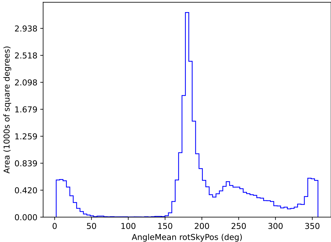
extra_ss_neo7_v3.4_10yrs All sky all bands: AngleMean rotSkyPos
