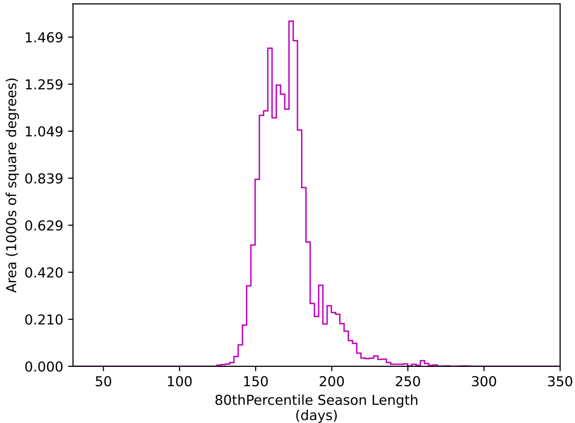
extra_ss_neo7_v3.4_10yrs WFD z band: 80thPercentile Season Length
