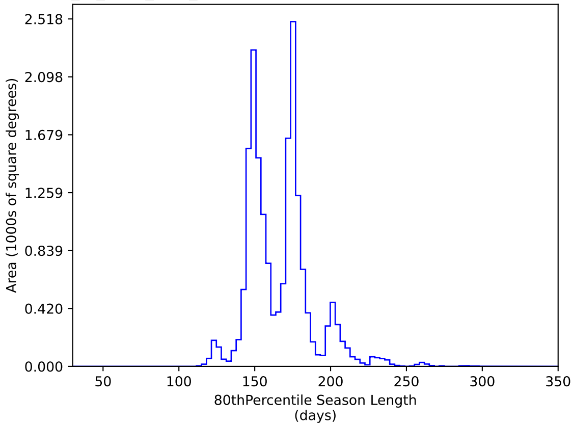
extra_ss_neo7_v3.4_10yrs WFD y band: 80thPercentile Season Length
