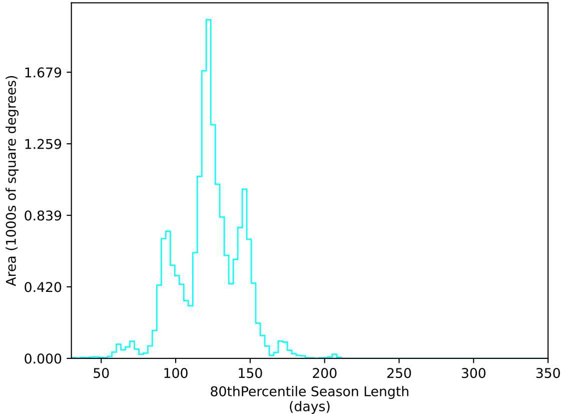
extra_ss_neo7_v3.4_10yrs WFD u band: 80thPercentile Season Length
