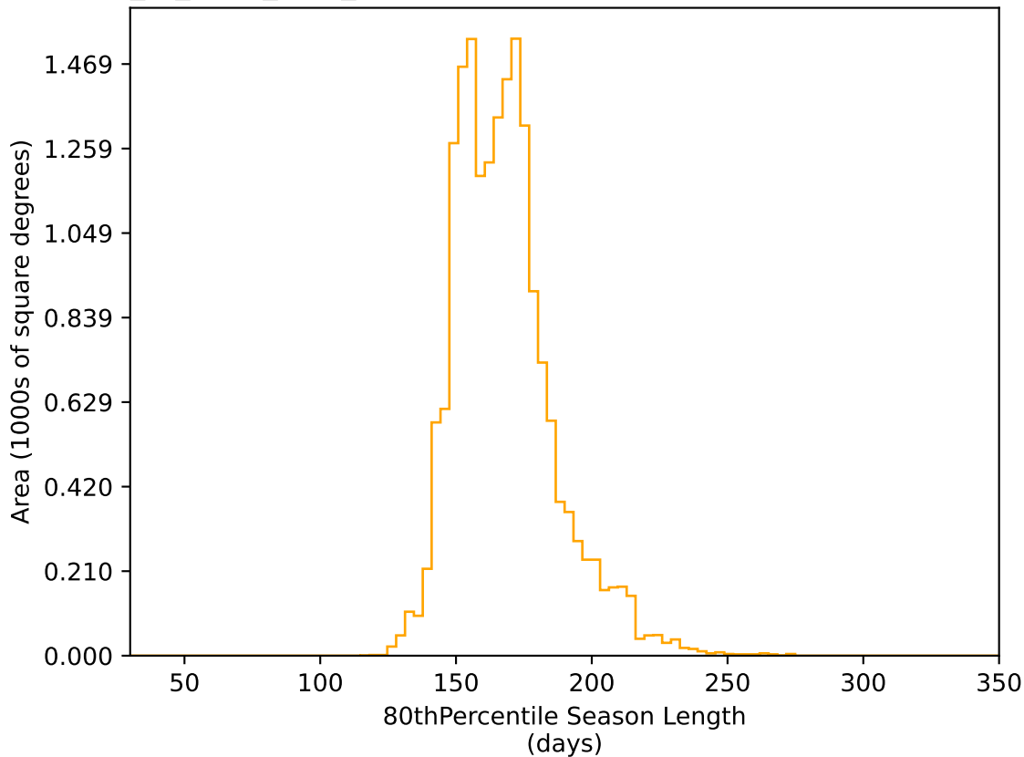
extra_ss_neo7_v3.4_10yrs WFD r band: 80thPercentile Season Length
