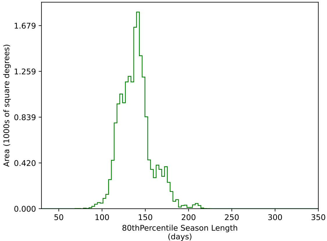
extra_ss_neo7_v3.4_10yrs WFD g band: 80thPercentile Season Length
