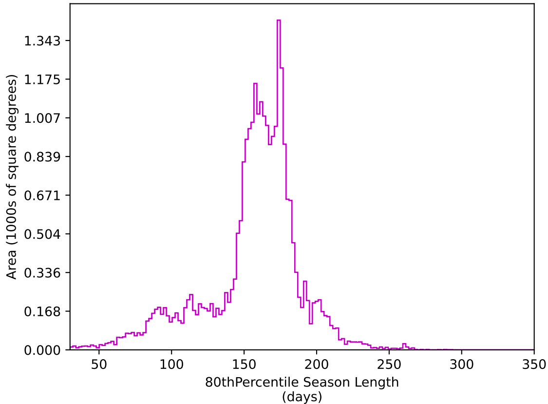
extra_ss_neo7_v3.4_10yrs All sky z band: 80thPercentile Season Length
