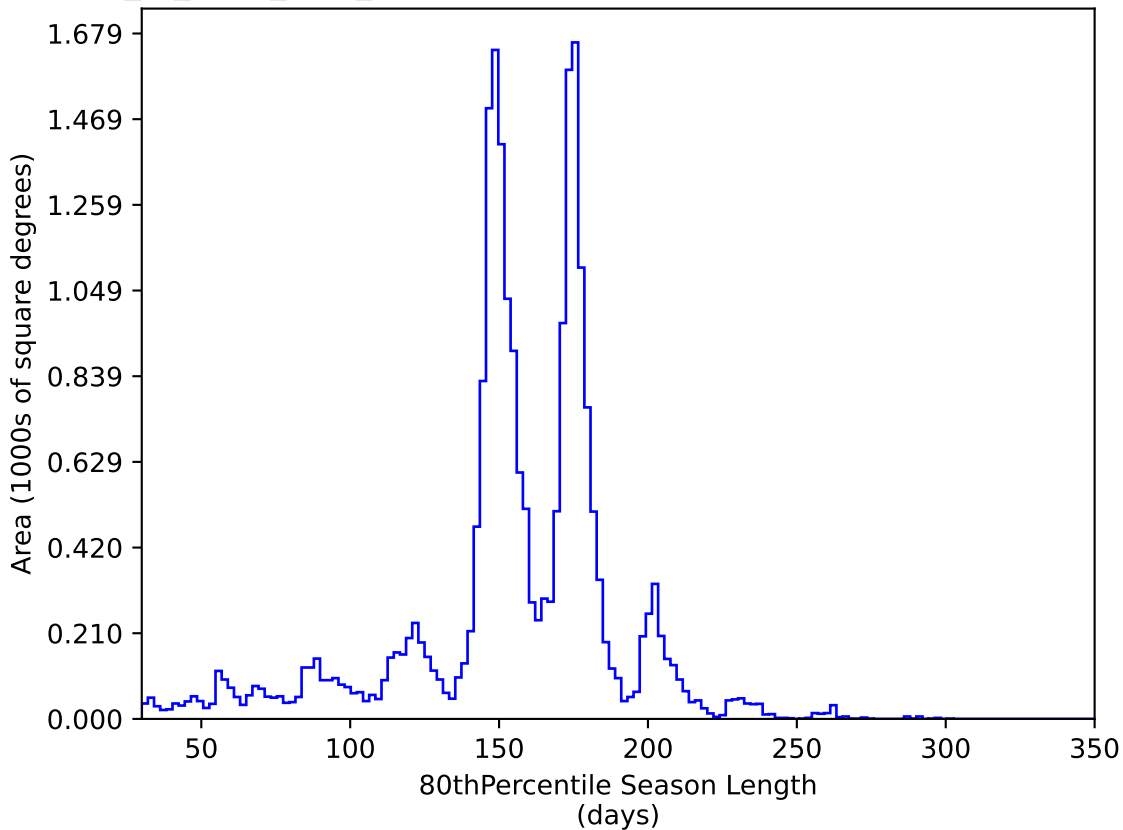
extra_ss_neo7_v3.4_10yrs All sky y band: 80thPercentile Season Length
