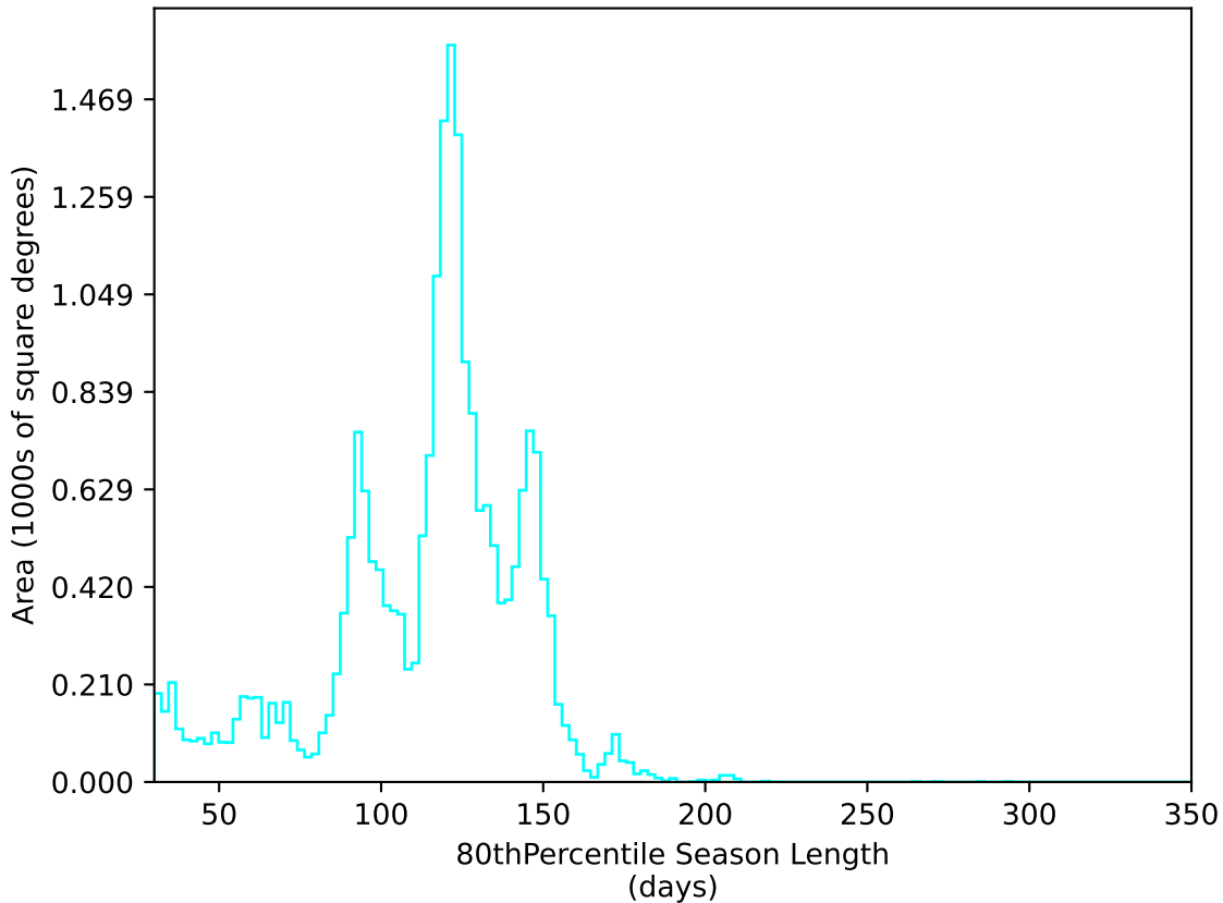
extra_ss_neo7_v3.4_10yrs All sky u band: 80thPercentile Season Length
