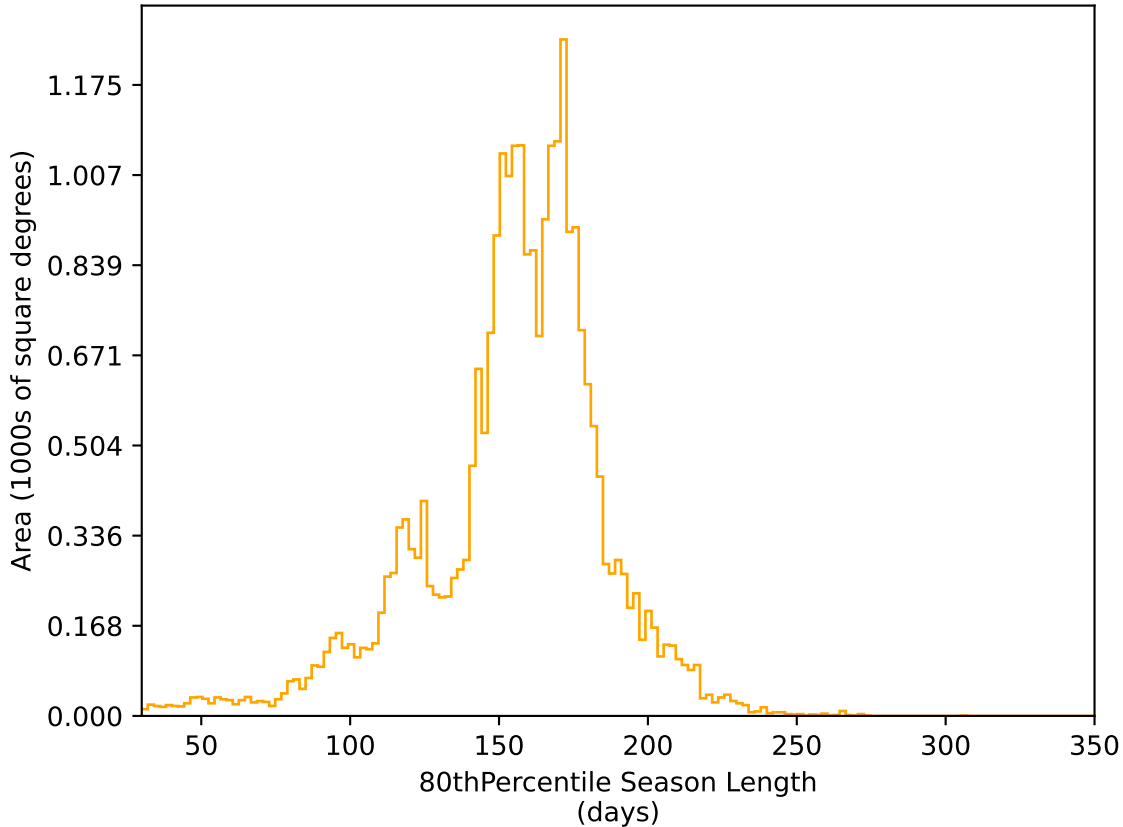
extra_ss_neo7_v3.4_10yrs All sky r band: 80thPercentile Season Length
