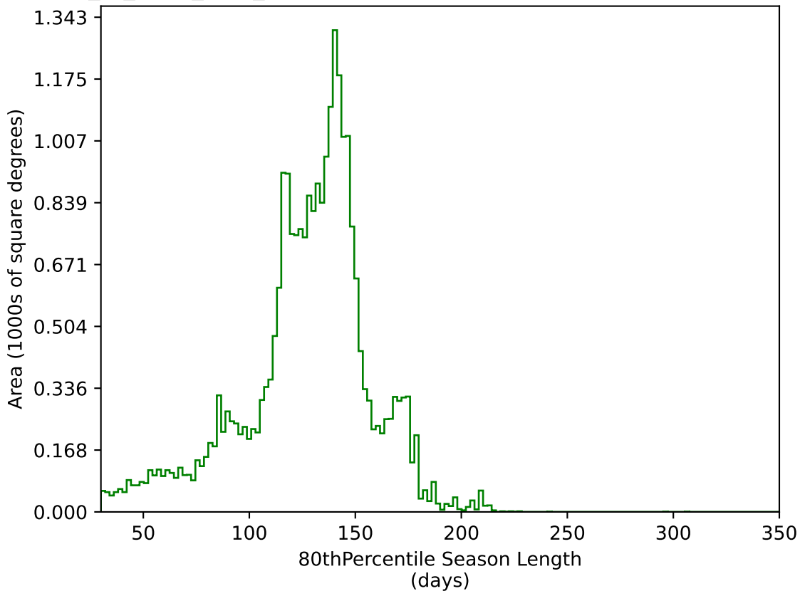
extra_ss_neo7_v3.4_10yrs All sky g band: 80thPercentile Season Length
