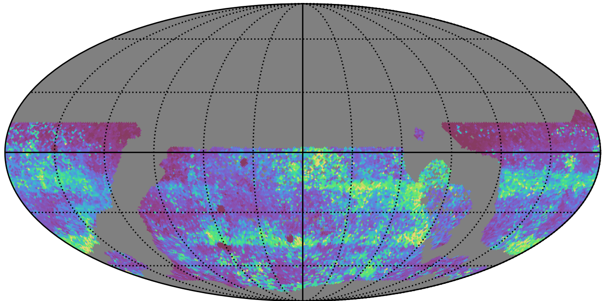
extra_ss_neo7_v3.4_10yrs WFD zy bands: 75th Percentile Intranight Timespan
