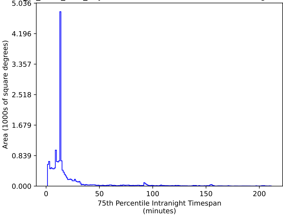
extra_ss_neo7_v3.4_10yrs WFD z band: 75th Percentile Intranight Timespan
