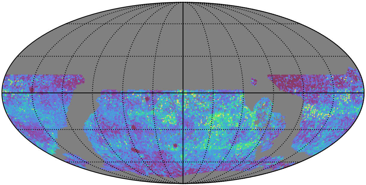
extra_ss_neo7_v3.4_10yrs WFD y band: 75th Percentile Intranight Timespan
