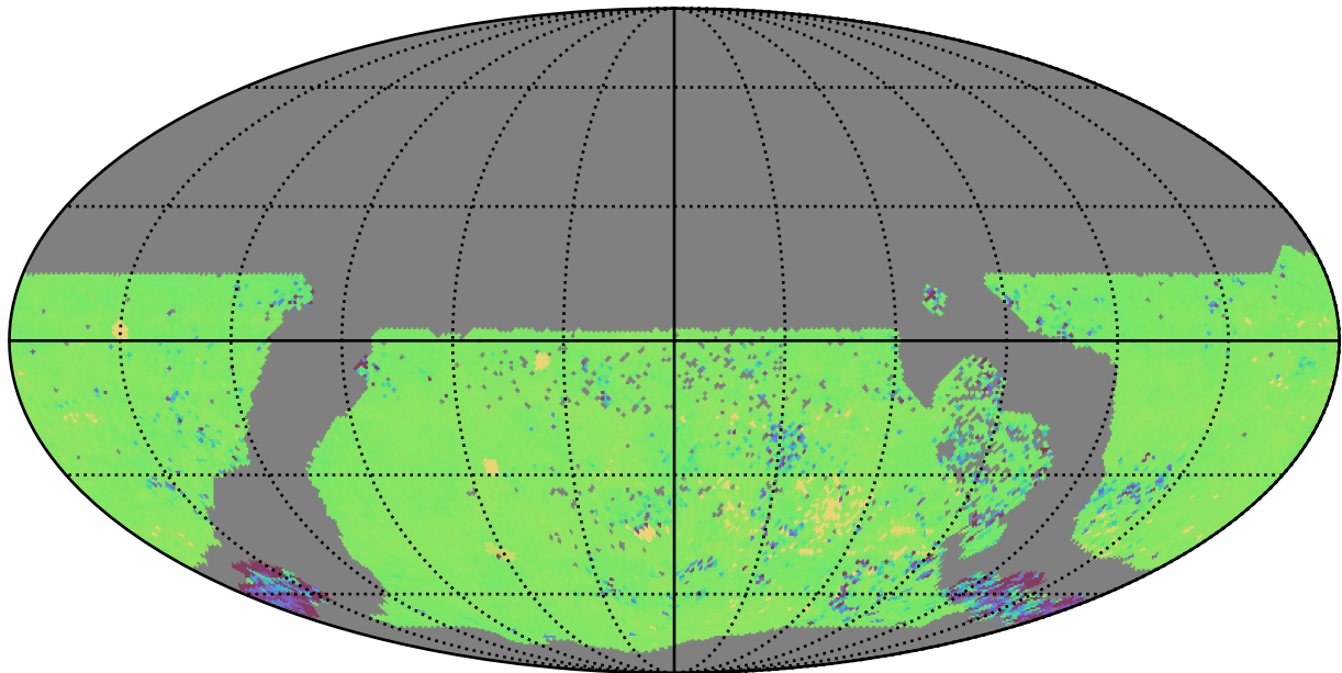
extra_ss_neo7_v3.4_10yrs WFD ug bands: 75th Percentile Intranight Timespan
