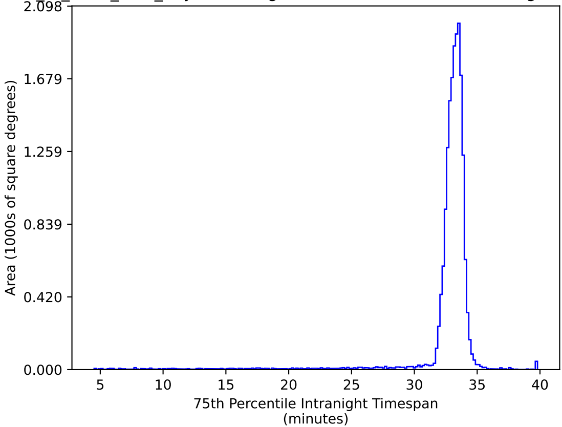
extra_ss_neo7_v3.4_10yrs WFD ug bands: 75th Percentile Intranight Timespan
