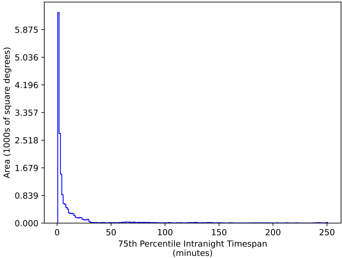
extra_ss_neo7_v3.4_10yrs WFD u band: 75th Percentile Intranight Timespan
