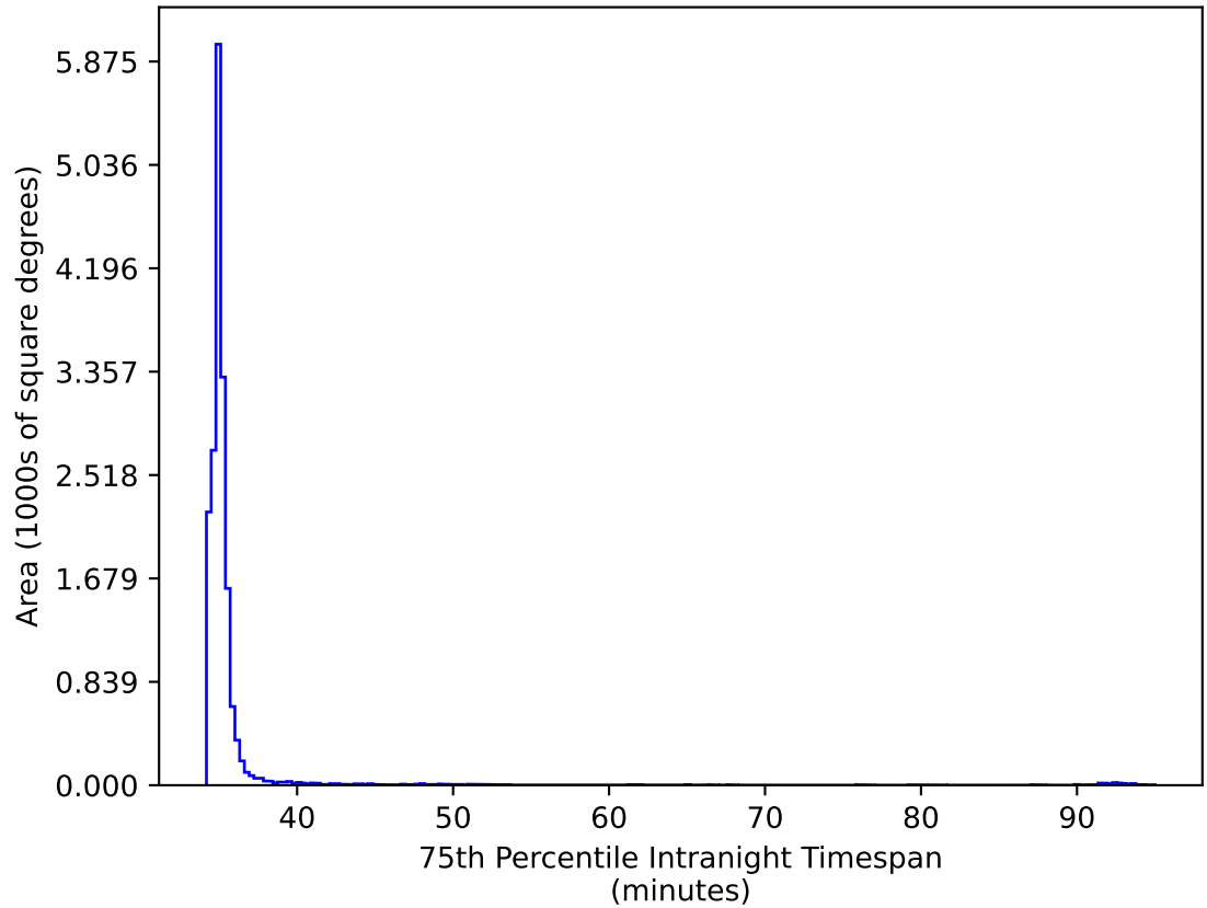
extra_ss_neo7_v3.4_10yrs WFD ri bands: 75th Percentile Intranight Timespan
