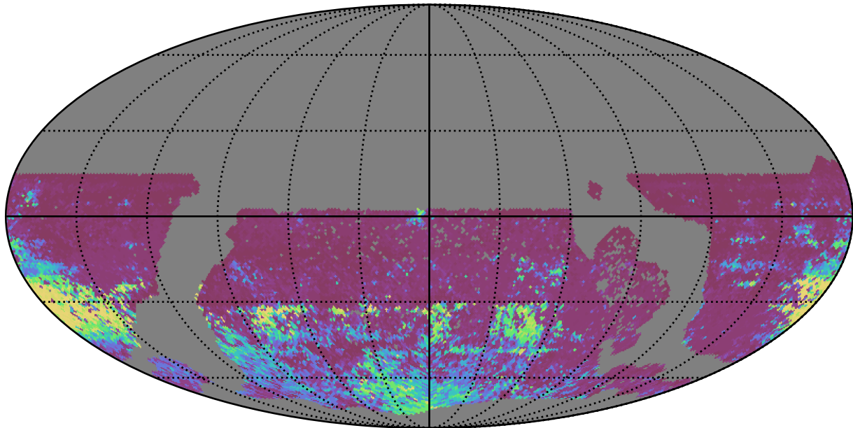
extra_ss_neo7_v3.4_10yrs WFD r band: 75th Percentile Intranight Timespan
