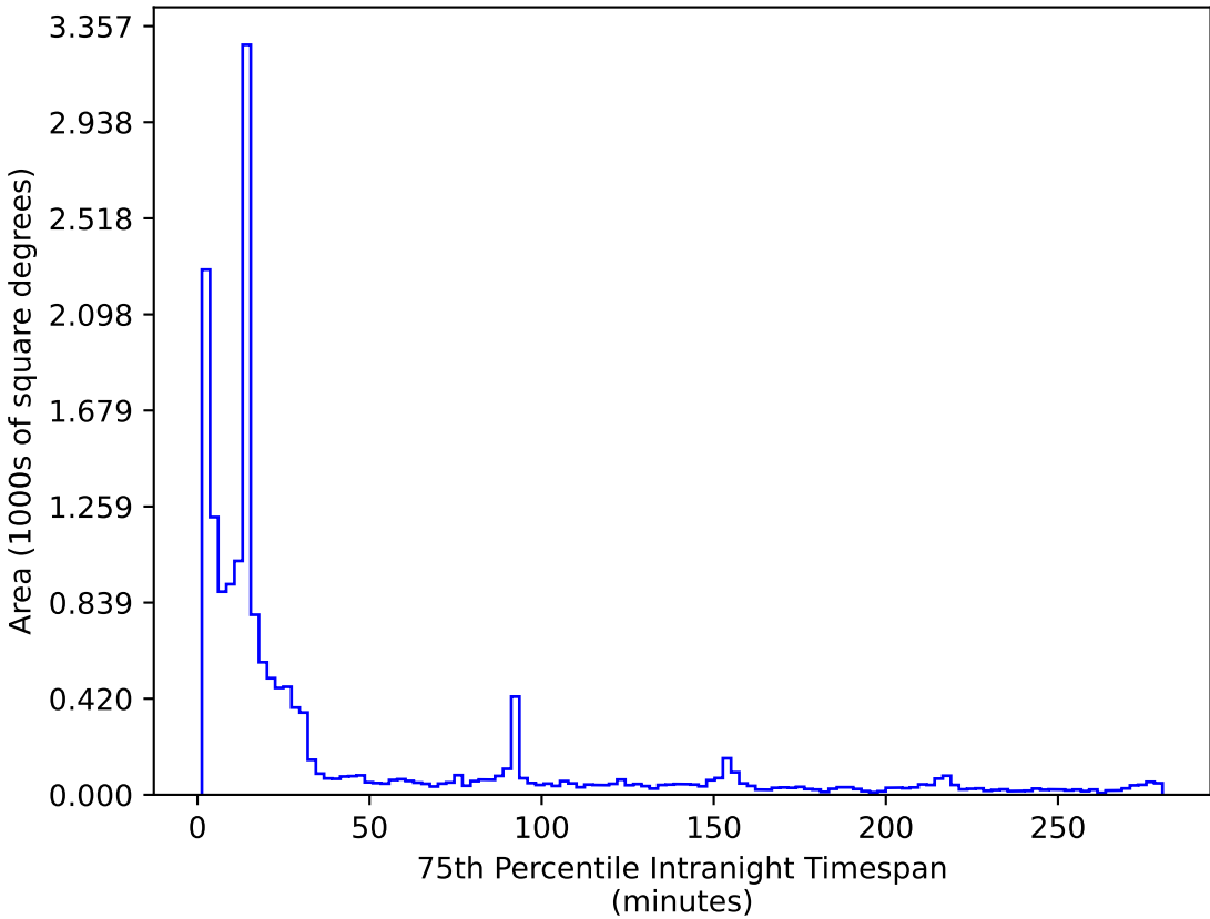
extra_ss_neo7_v3.4_10yrs WFD r band: 75th Percentile Intranight Timespan
