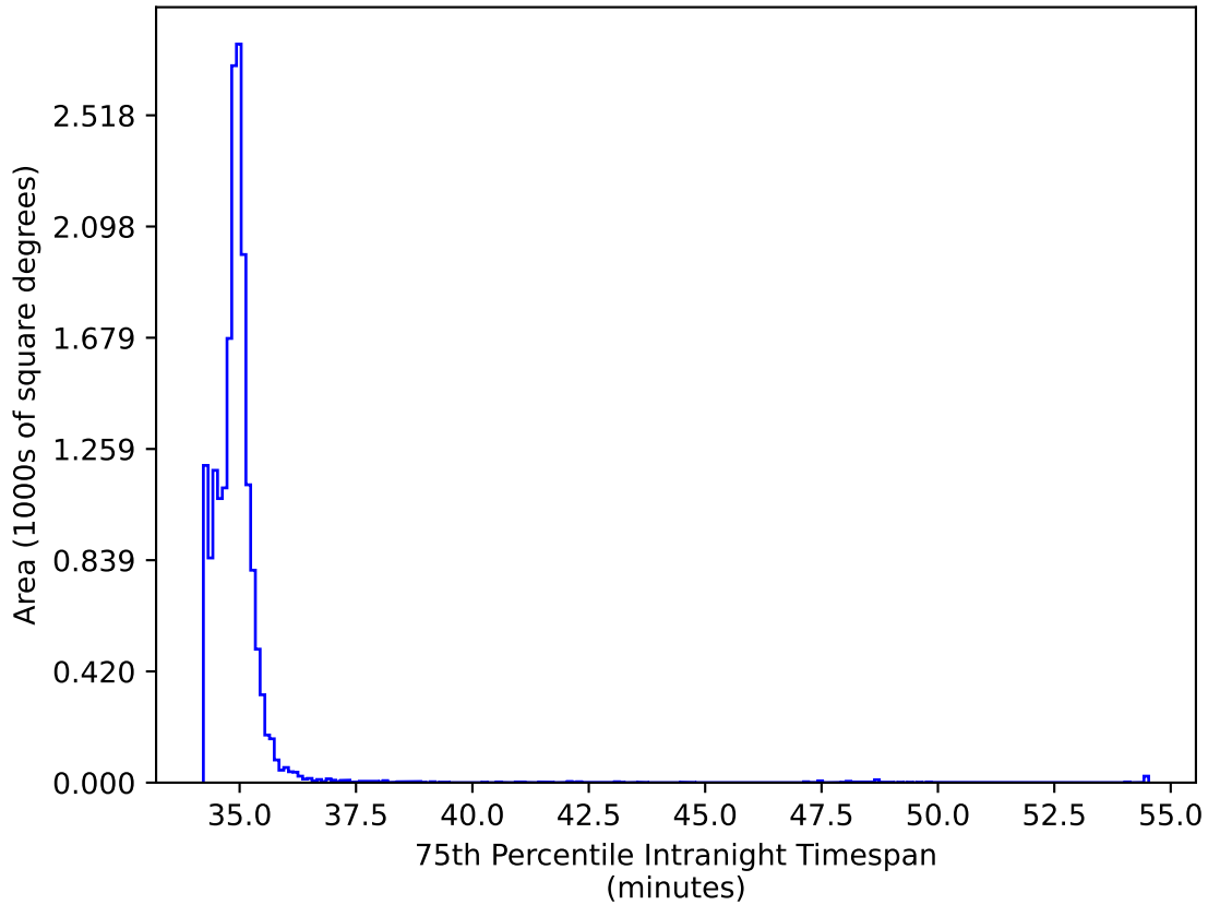
extra_ss_neo7_v3.4_10yrs WFD iz bands: 75th Percentile Intranight Timespan
