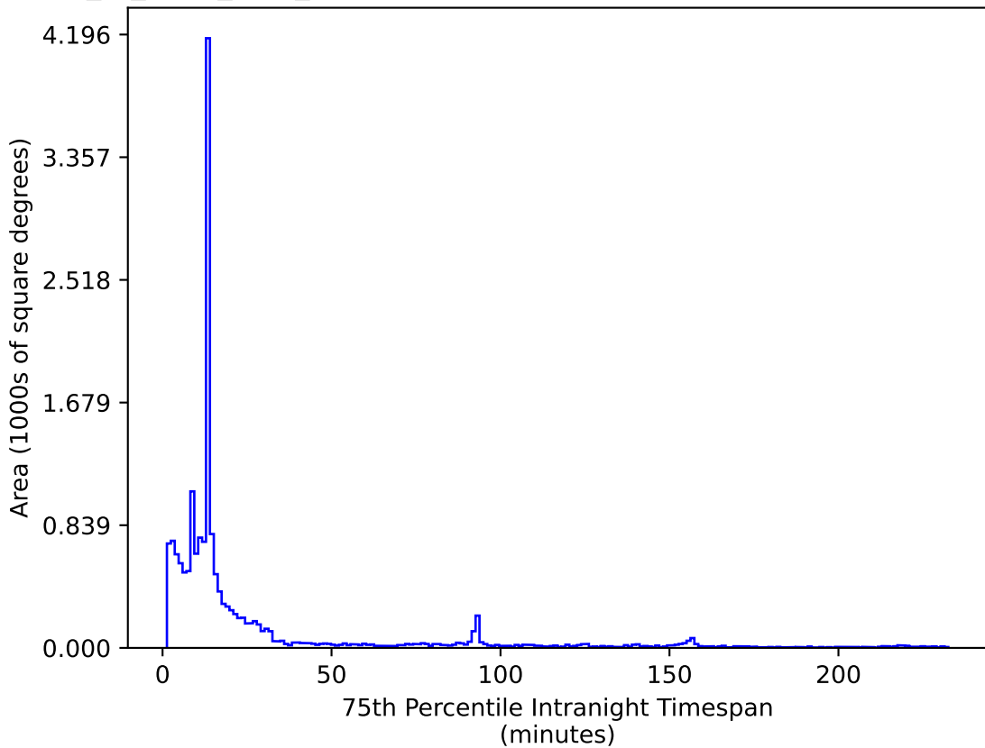
extra_ss_neo7_v3.4_10yrs WFD i band: 75th Percentile Intranight Timespan
