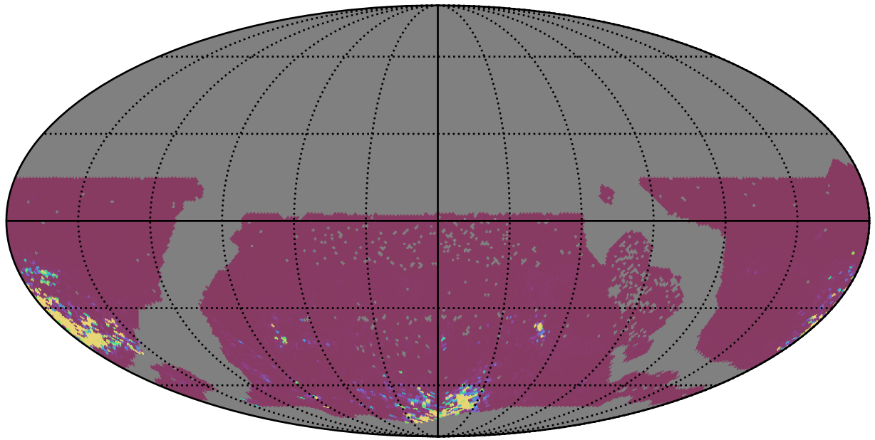
extra_ss_neo7_v3.4_10yrs WFD gr bands: 75th Percentile Intranight Timespan
