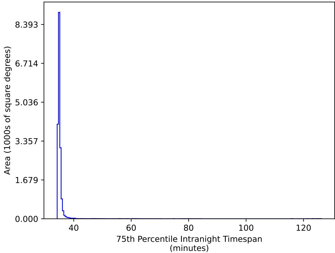
extra_ss_neo7_v3.4_10yrs WFD gr bands: 75th Percentile Intranight Timespan
