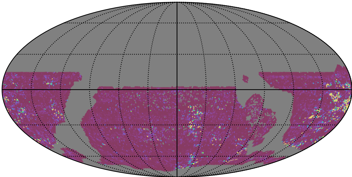
extra_ss_neo7_v3.4_10yrs WFD g band: 75th Percentile Intranight Timespan
