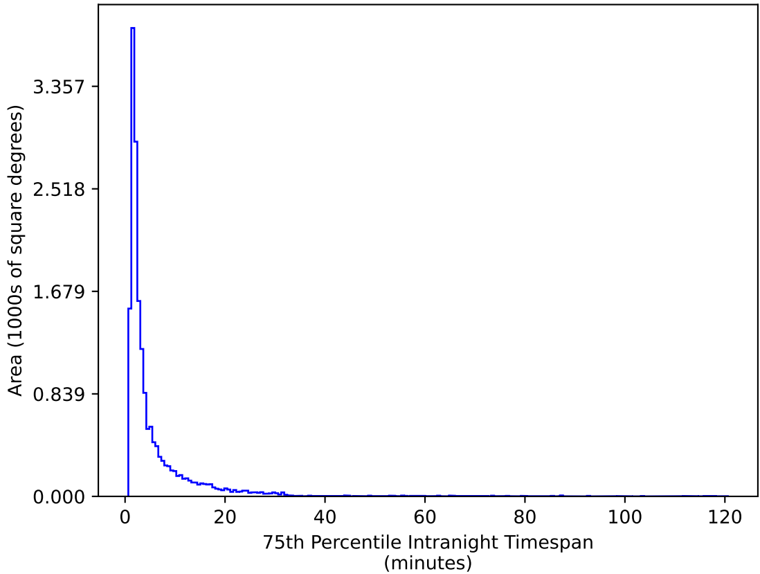
extra_ss_neo7_v3.4_10yrs WFD g band: 75th Percentile Intranight Timespan
