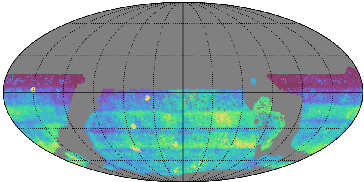
extra_ss_neo7_v3.4_10yrs WFD all bands: 75th Percentile Intranight Timespan
