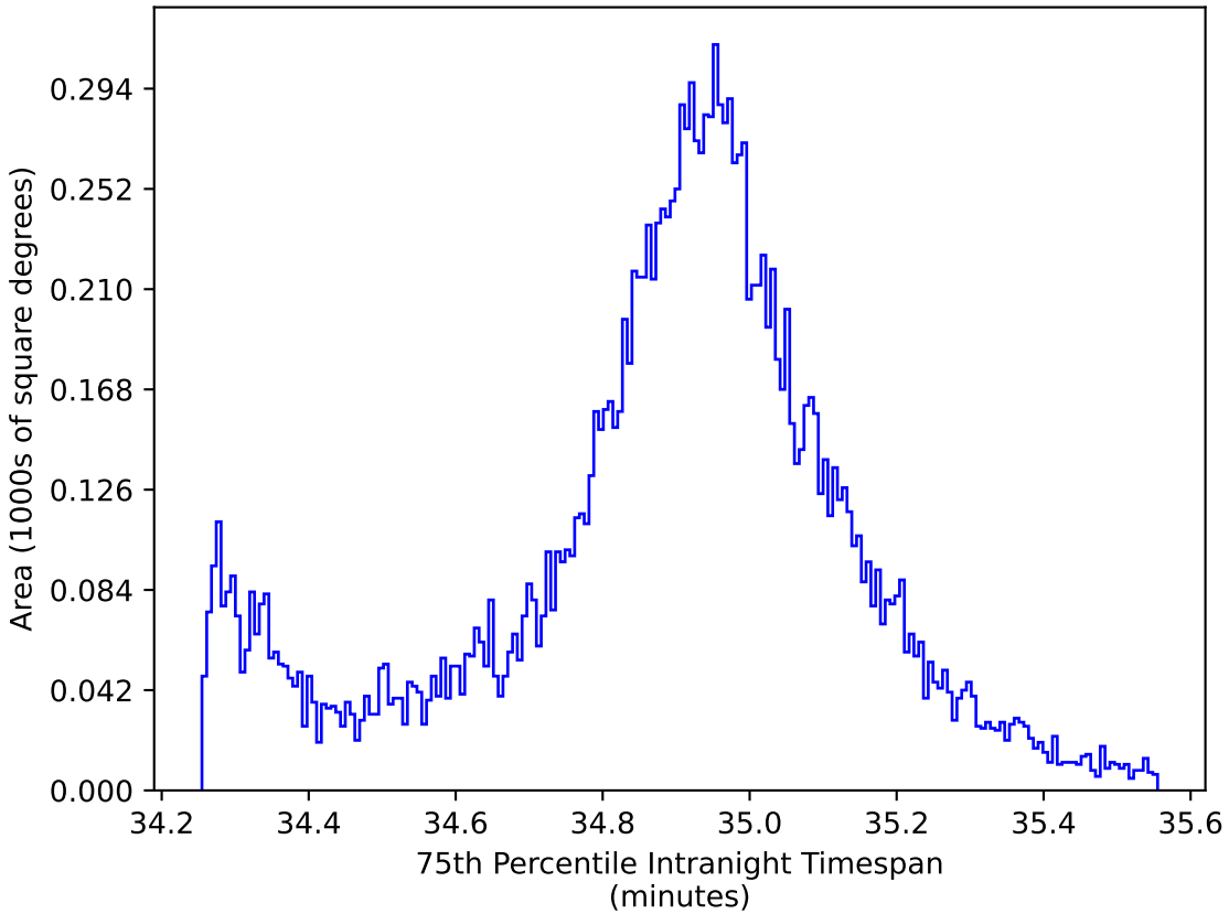
extra_ss_neo7_v3.4_10yrs WFD: 75th Percentile Intranight Timespan
