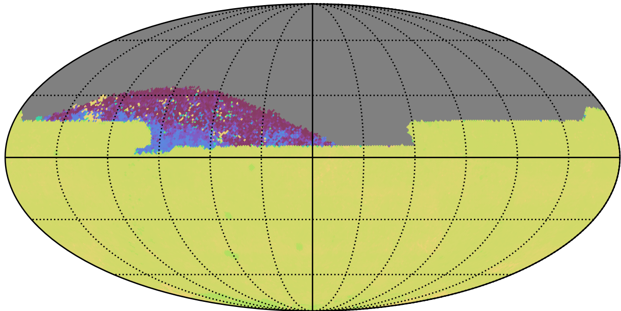
extra_ss_neo7_v3.4_10yrs All sky zy bands: 75th Percentile Intranight Timespan
