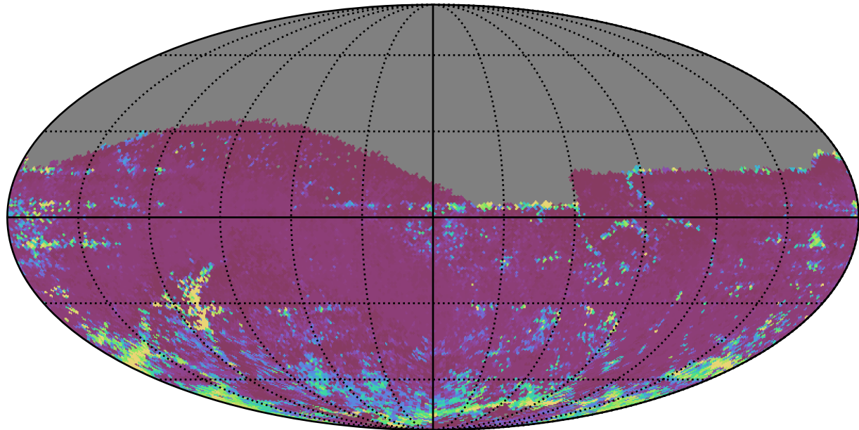
extra_ss_neo7_v3.4_10yrs All sky z band: 75th Percentile Intranight Timespan
