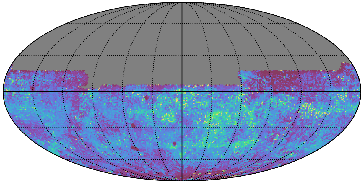
extra_ss_neo7_v3.4_10yrs All sky y band: 75th Percentile Intranight Timespan
