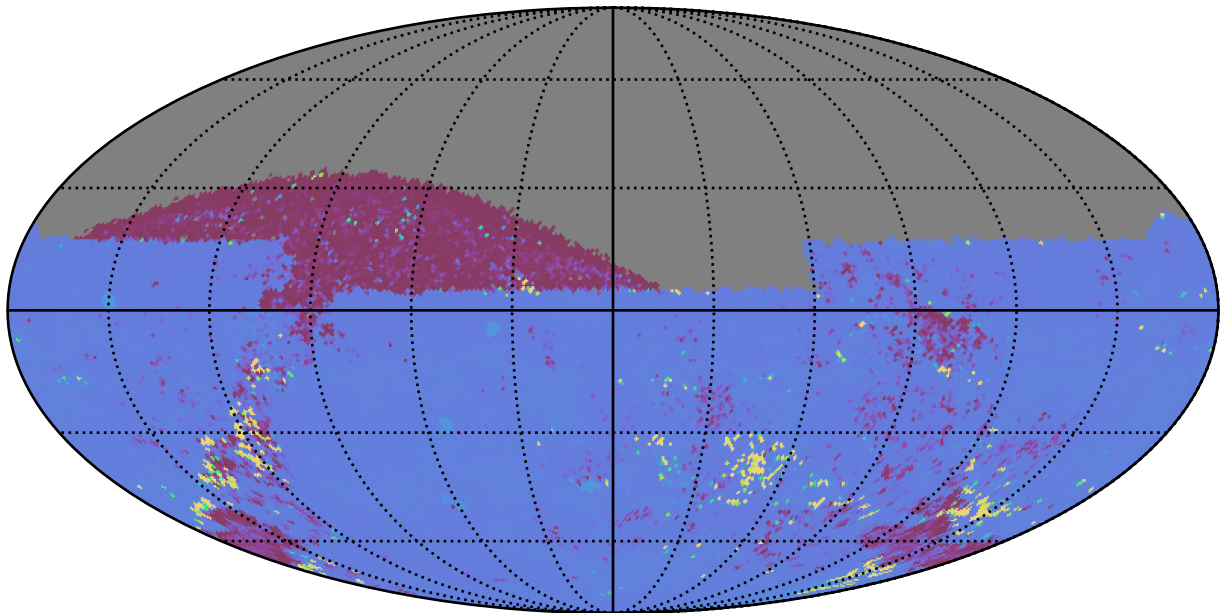
extra_ss_neo7_v3.4_10yrs All sky ug bands: 75th Percentile Intranight Timespan
