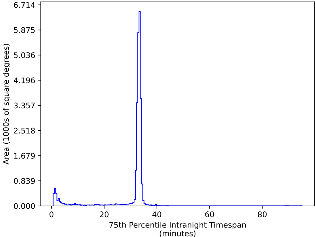
extra_ss_neo7_v3.4_10yrs All sky ug bands: 75th Percentile Intranight Timespan
