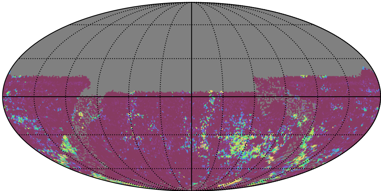
extra_ss_neo7_v3.4_10yrs All sky u band: 75th Percentile Intranight Timespan
