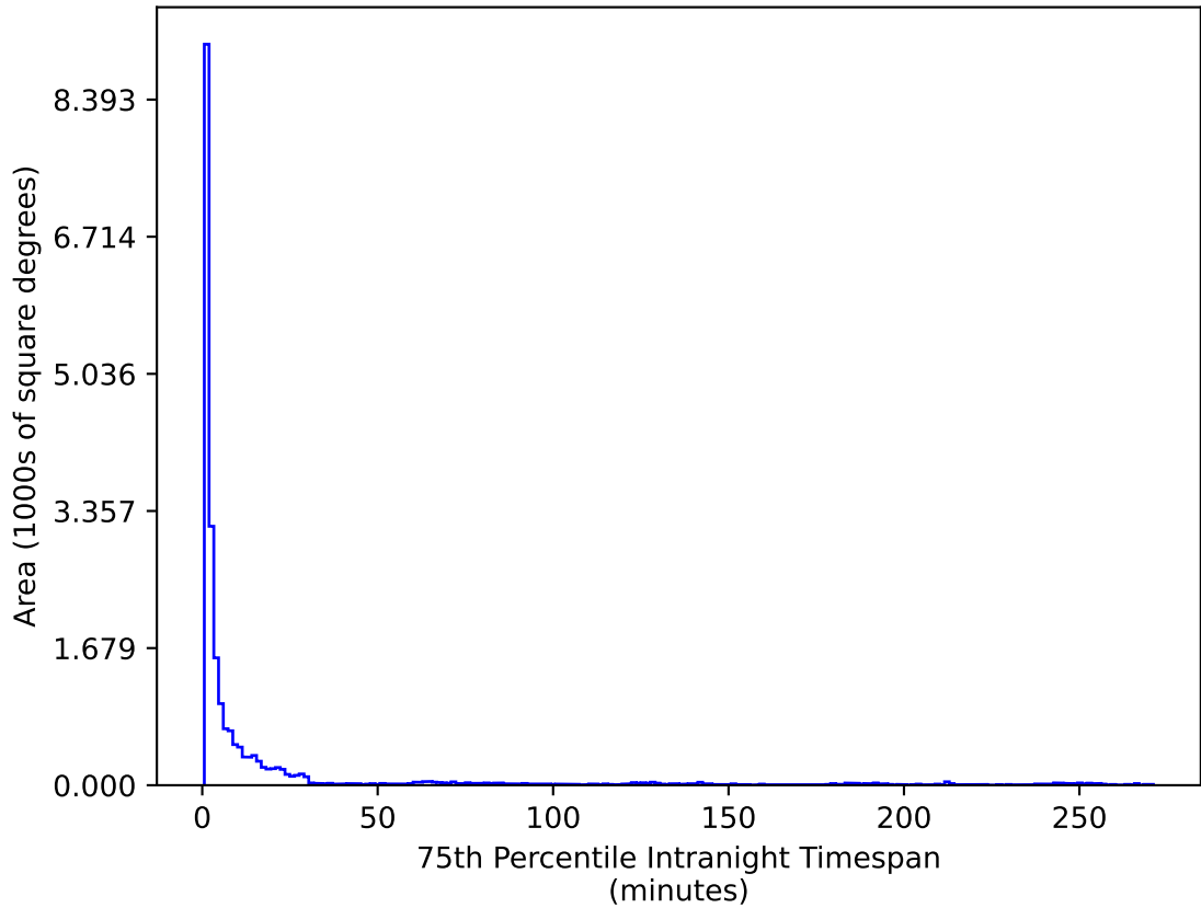
extra_ss_neo7_v3.4_10yrs All sky u band: 75th Percentile Intranight Timespan
