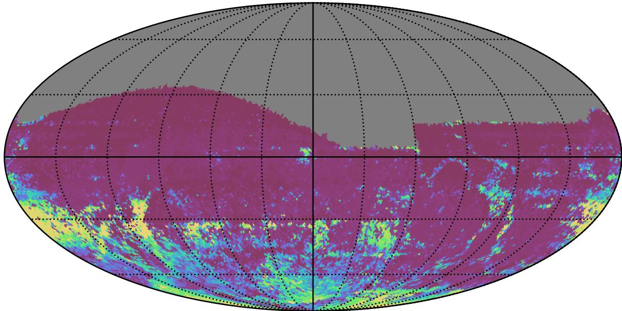
extra_ss_neo7_v3.4_10yrs All sky r band: 75th Percentile Intranight Timespan
