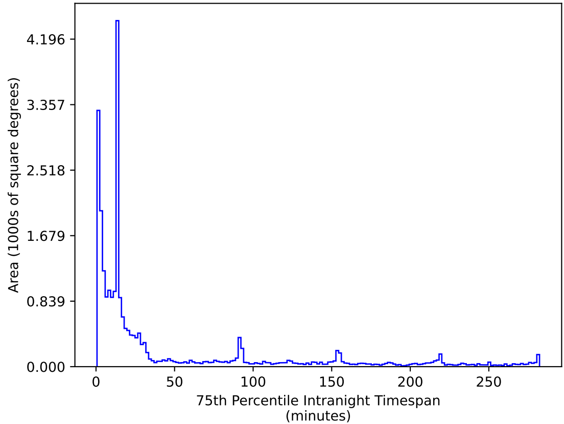
extra_ss_neo7_v3.4_10yrs All sky r band: 75th Percentile Intranight Timespan
