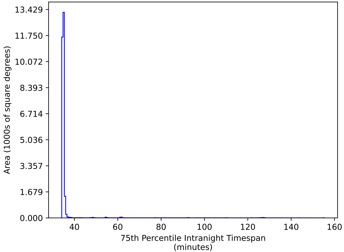
extra_ss_neo7_v3.4_10yrs All sky iz bands: 75th Percentile Intranight Timespan
