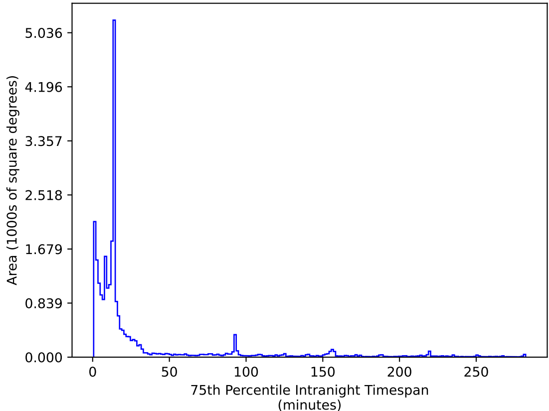
extra_ss_neo7_v3.4_10yrs All sky i band: 75th Percentile Intranight Timespan
