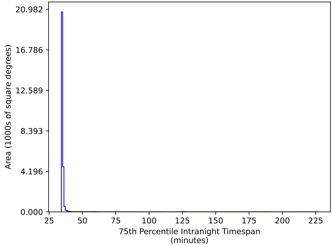
extra_ss_neo7_v3.4_10yrs All sky gr bands: 75th Percentile Intranight Timespan
