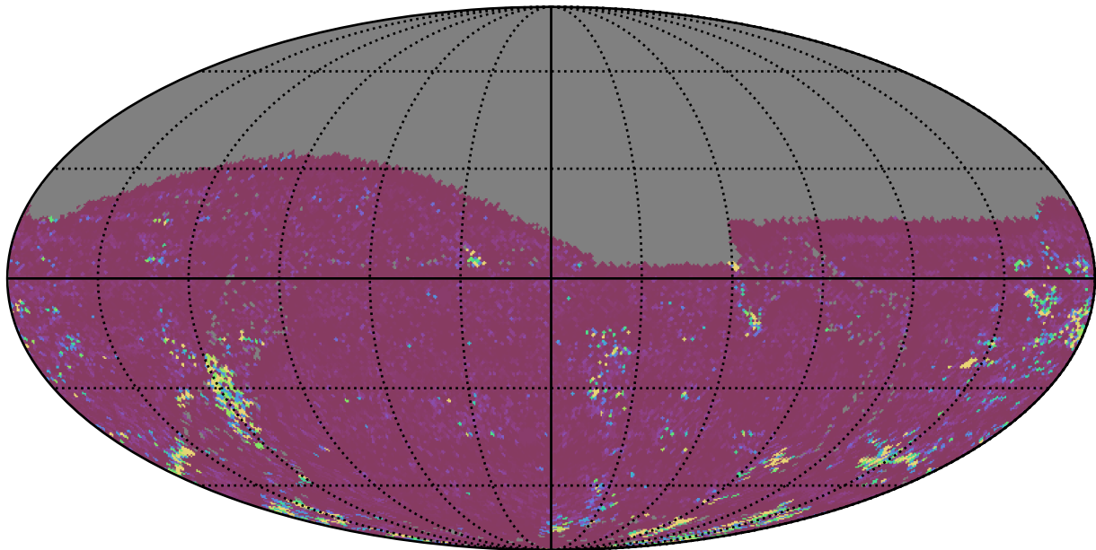
extra_ss_neo7_v3.4_10yrs All sky g band: 75th Percentile Intranight Timespan
