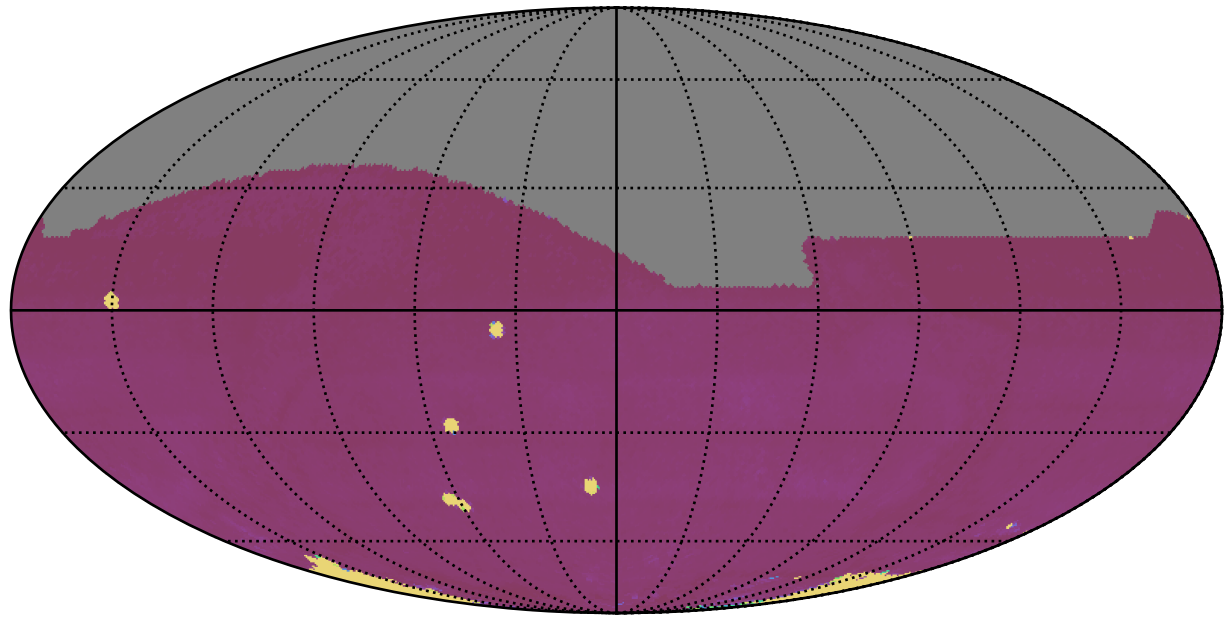
extra_ss_neo7_v3.4_10yrs All sky all bands: 75th Percentile Intranight Timespan
