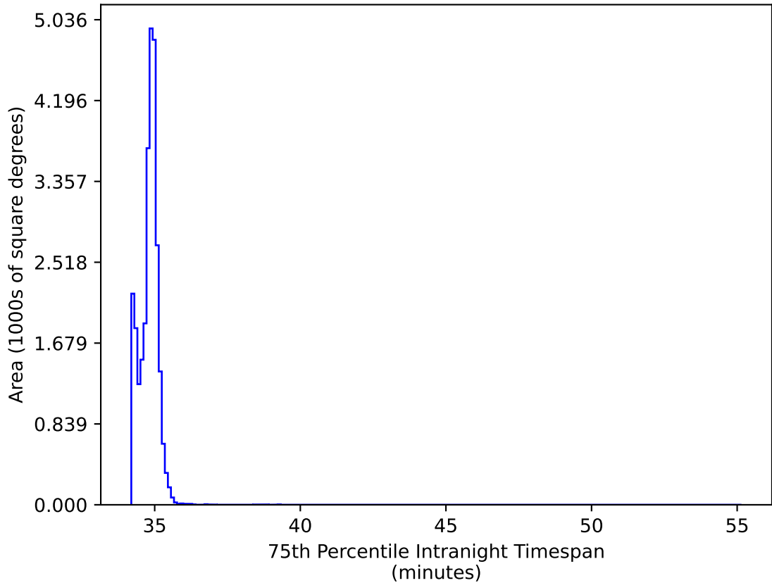
extra_ss_neo7_v3.4_10yrs All sky all bands: 75th Percentile Intranight Timespan
