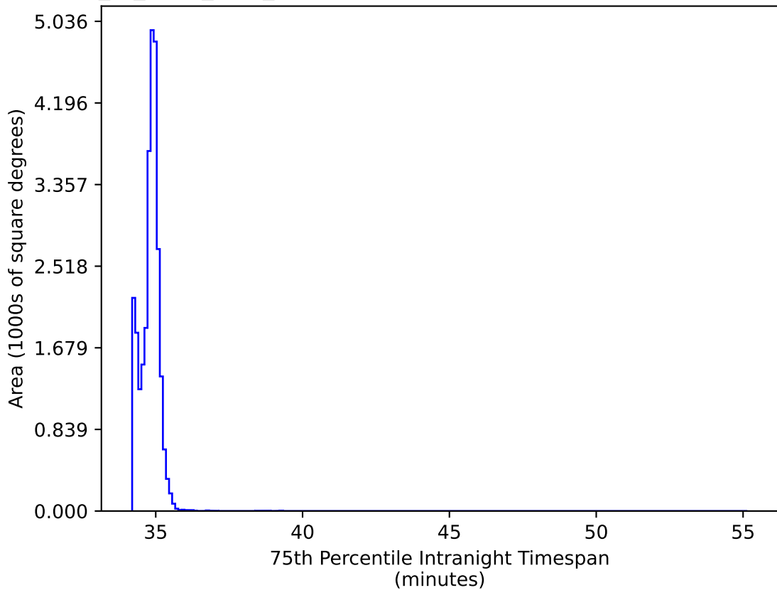
extra_ss_neo7_v3.4_10yrs All sky: 75th Percentile Intranight Timespan
