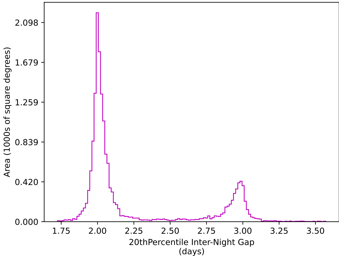
extra_ss_neo7_v3.4_10yrs WFD z band: 20thPercentile Inter-Night Gap
