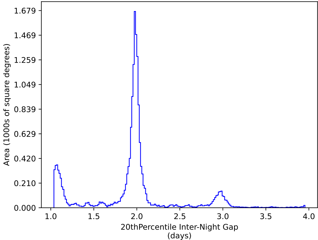
extra_ss_neo7_v3.4_10yrs WFD y band: 20thPercentile Inter-Night Gap
